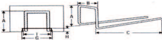
STABOX TYPE 160D (No. 4 or 5 rebar)
