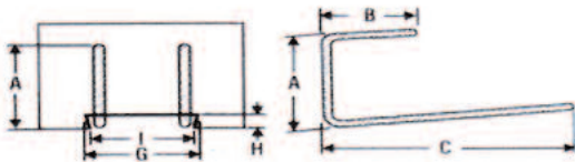
STABOX TYPE 160DD (No. 4 or 5 rebar)
